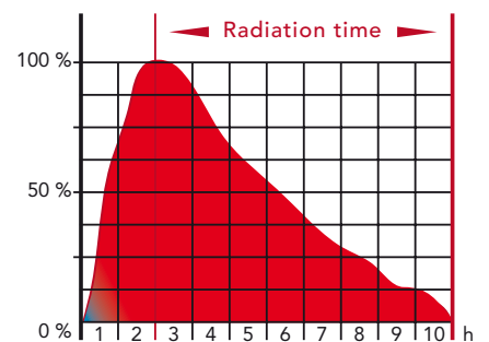
Radiation time with charge of 6 kg wood without adding of other fuels.
